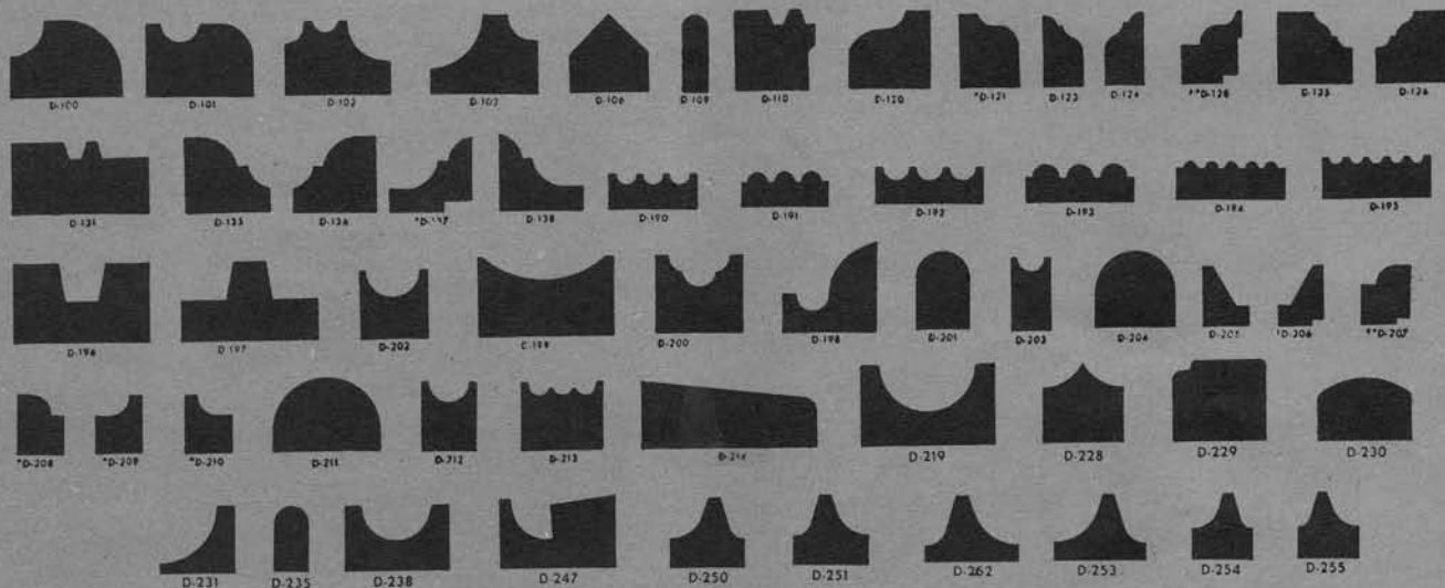
Three lip cutter (Available with profiles as shown)
