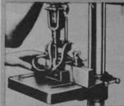
Drill square holes. This mortising operation is needed for door and screen construction and repair.
