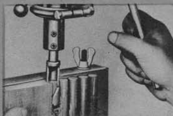
Cut your own plugs and dowels.
