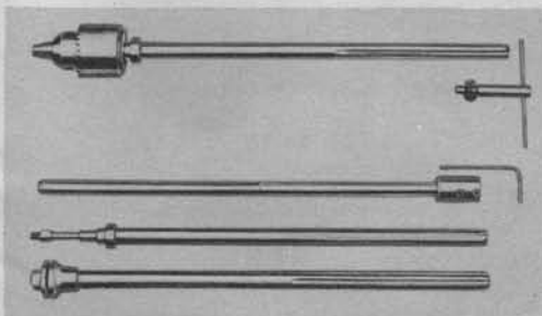
Interchangeable spindles mean fast cutting tool changes—no pulling, prying or hammering on chuck—and there's a "right" spindle for every job.
