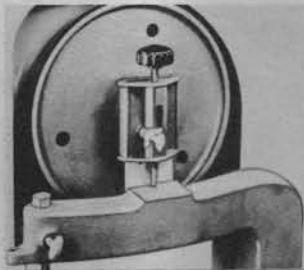
Wheel tensions and blade tracking adjustments on upper arm casting. Handy accurate means of correcting alignments of blade, ... keeping correct tension at all times.
