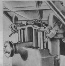
Heavy trunnions and solid under table construction—makes table surface rigid and firm.
