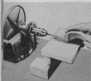
Horizontal drilling, using a keyless chuck . . . allows you to end-drill extremely long pieces.
