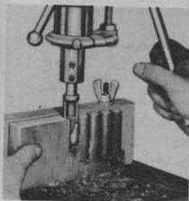
Cutting short dowels or plugs for cabinet or other work is a handy and easy operation.
