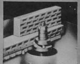
Cut moulded shapes, beads, flutes, etc. — a wide variety of shaper cutters are available for your selection.
