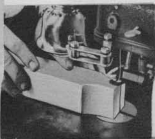
Big capacity cut! Up to 2" in wood, cuts to the center of a 32" panel. Variable speed pulley allows work in wood, metal or plastic!
