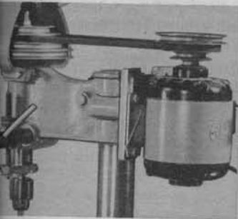
There are a full selection of speeds for drilling in wood, metal, plastic, glass and ceramics.
