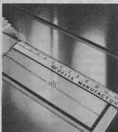
There is 11\frac{1}{2} " of table in front of blade—gives largest capacity work plenty of support.
