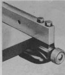
Delta self-aligning front fence clamp secures fence accurately with only one knob control.
