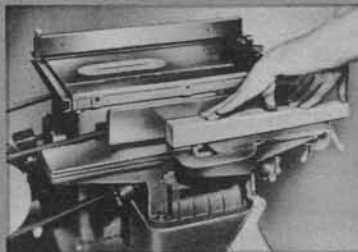
Taper cuts are easy: simply adjust the two table-sections to provide the wanted degree of taper.
